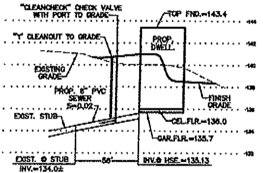
PROFILE - SCALE: Hor. 1" = 40' Vert. 1" = 4'
